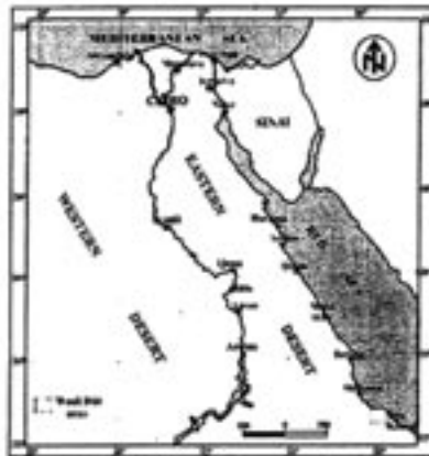
Fig. (1) Location map of Wadi Diit area, Southern Eastern Desert, Egypt.
