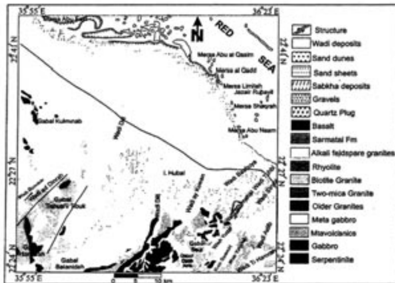
Fig. (2) Geologic map of Wadi Diit area, Southern Eastern Desert, Egypt
